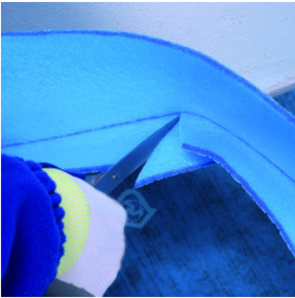
Cut the lower part of Mapesilent Band R to form a 90° angle in correspondence with the angles
